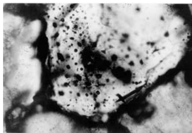
Photo 7. Pale-green sphalerite with primary growth zones defined by liquid-rich and vapour-rich fluid inclusions, Torbrit deposit. Sample RP-T-1. Transmitted plane light. Long field of view is 375 \mu\text{m} .
